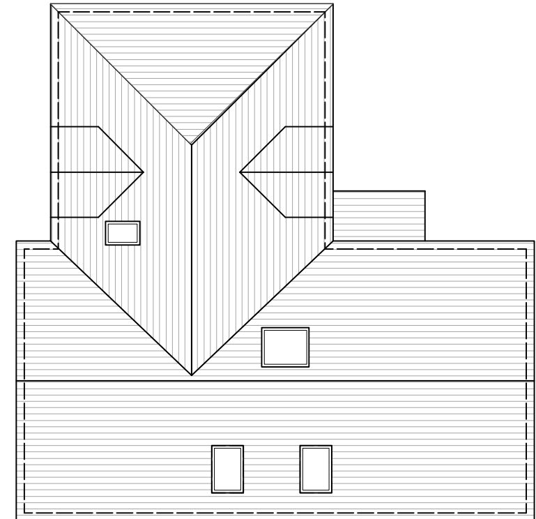
Roof Plan
