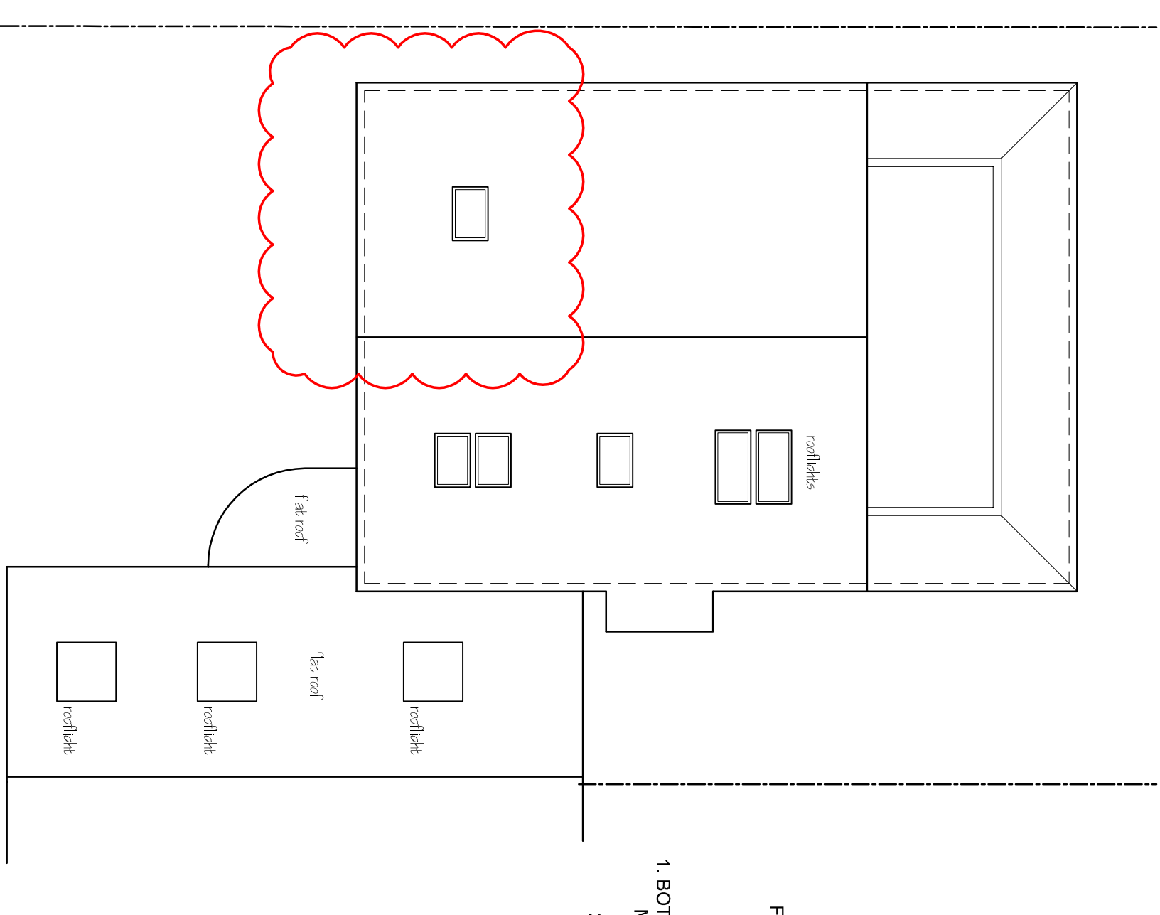
Roof 1:100
