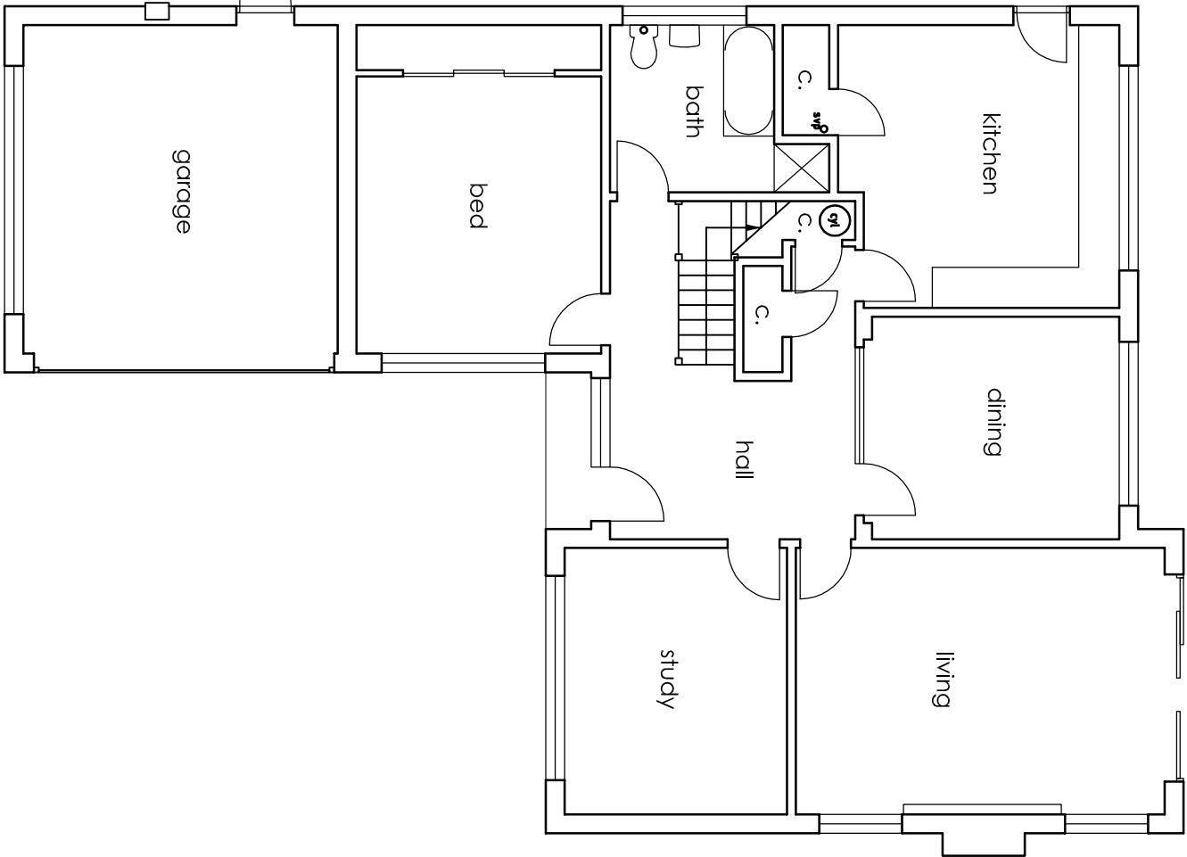
Ground 1:100
