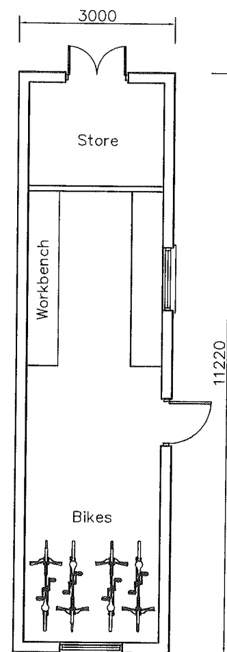
PLAN
