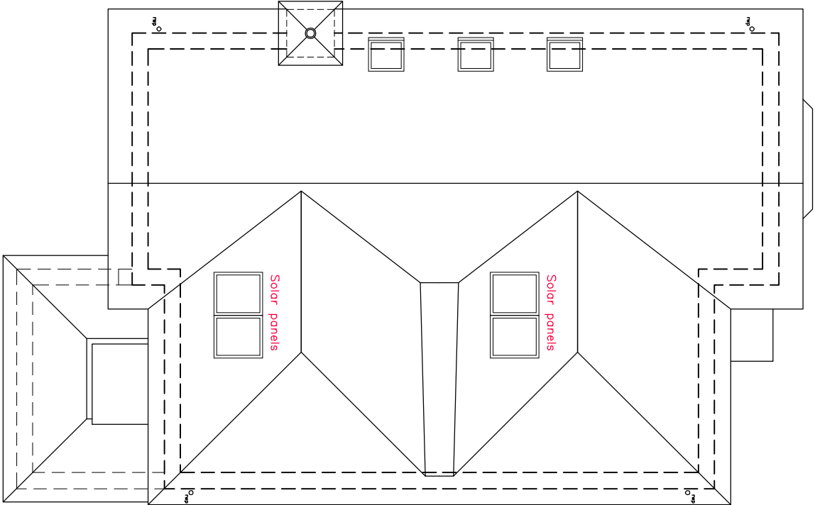
Roof Plan
