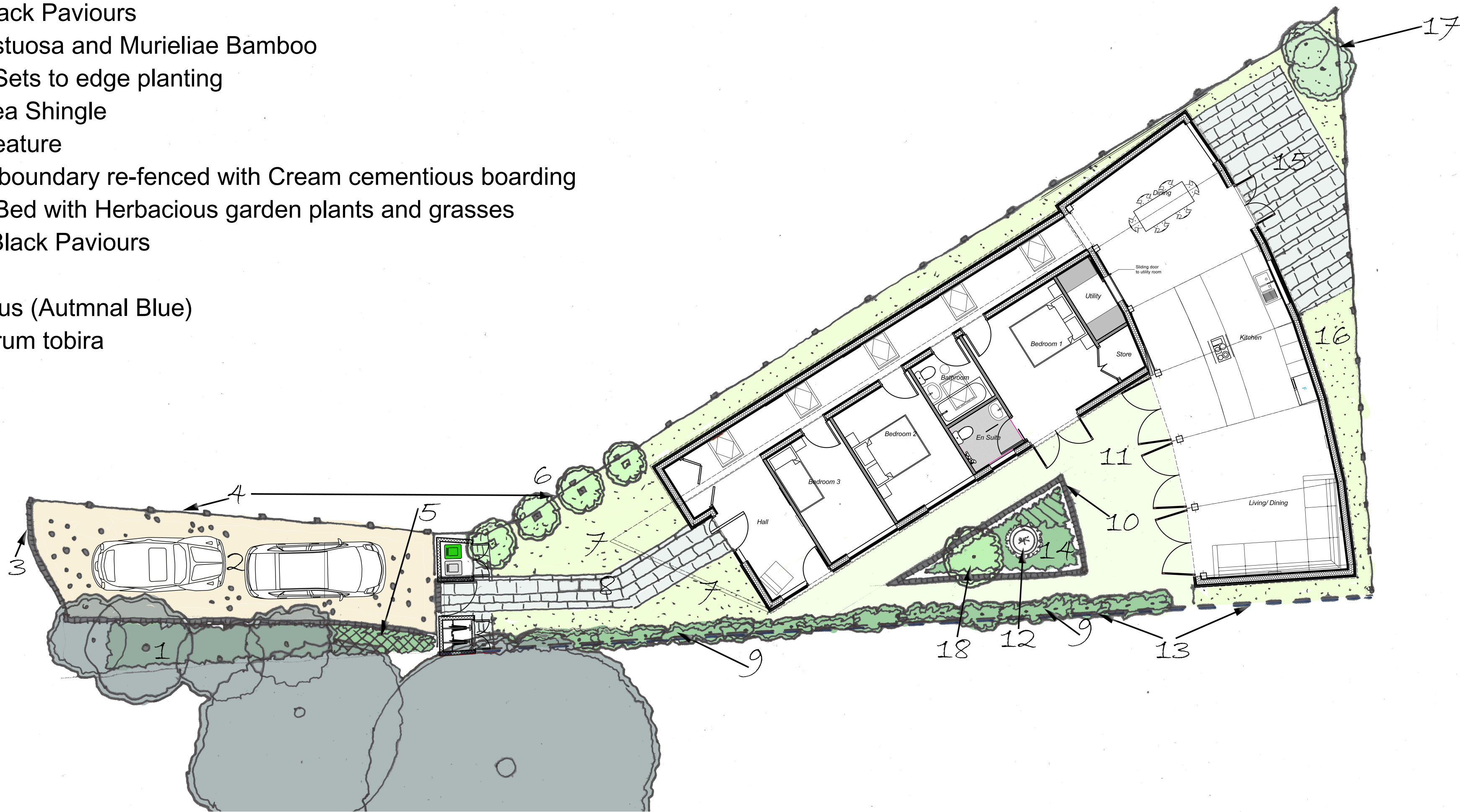
Landscaping Plan
