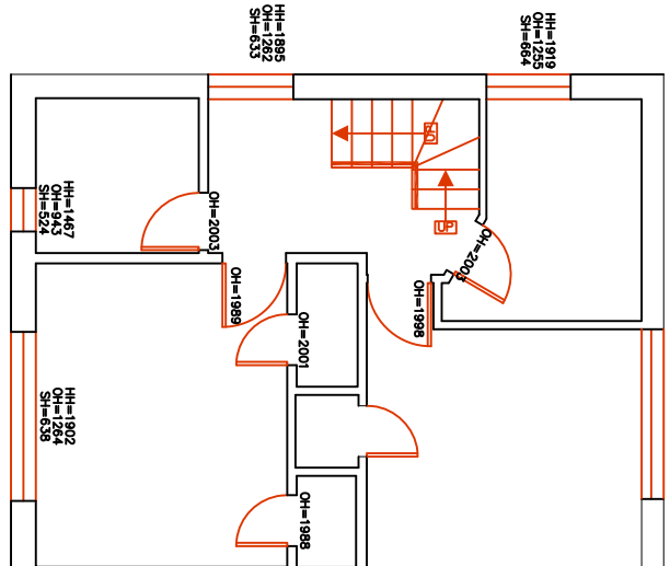
Existing first floor plan 1:100
