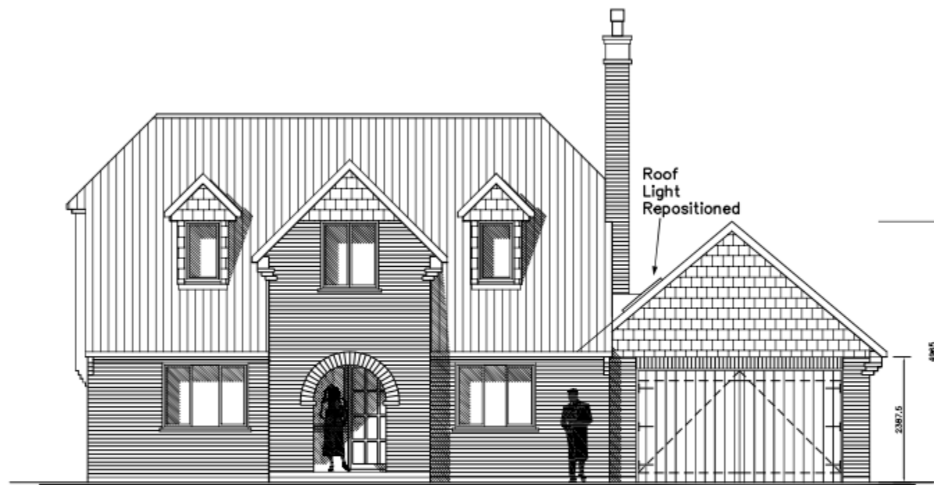
NORTH
