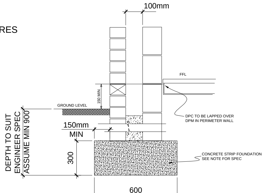
STRIP FOUNDATION DETAIL NOT TO SCALE
