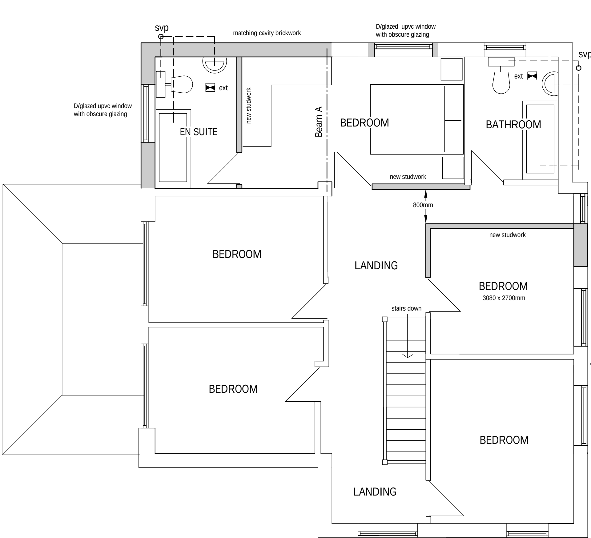
Prop. First Floor Plan 1 : 50
