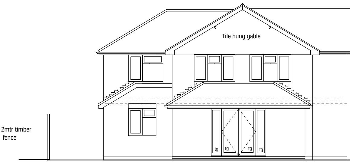
Ext'g Side Elevation
