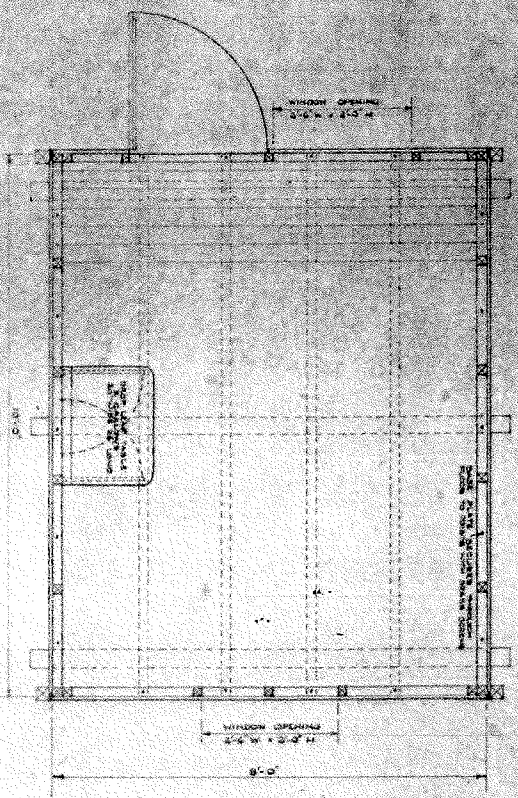
FLOOR PLAN
