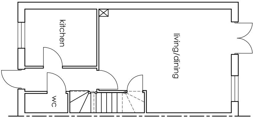
Ground 1:100
