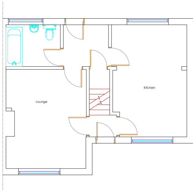
Existing Ground Floor
