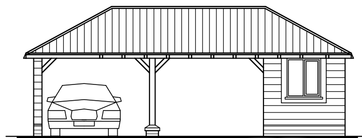
WEST ELEVATION
