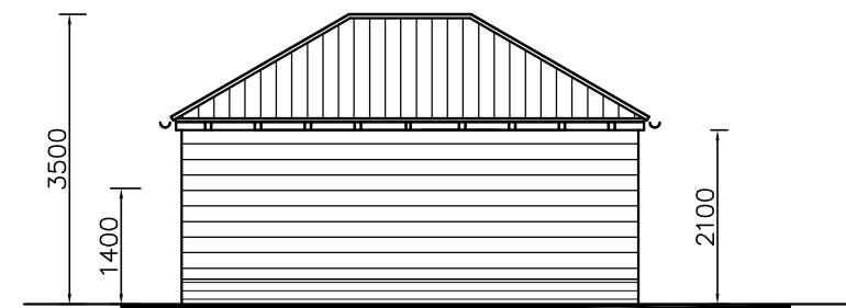
SOUTH ELEVATION
