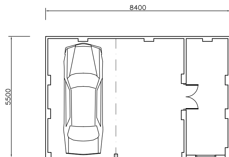
PLAN
