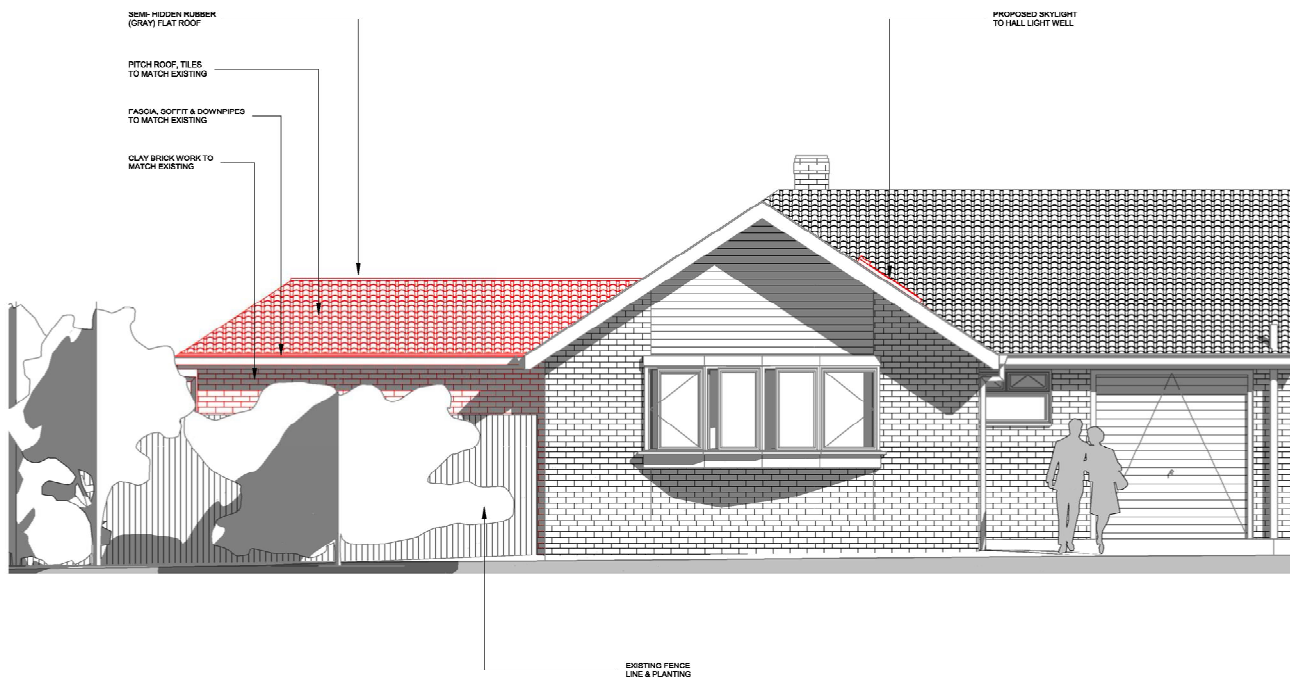
DETAILED EAST ELEVATION (FRONT) 1 : 50
