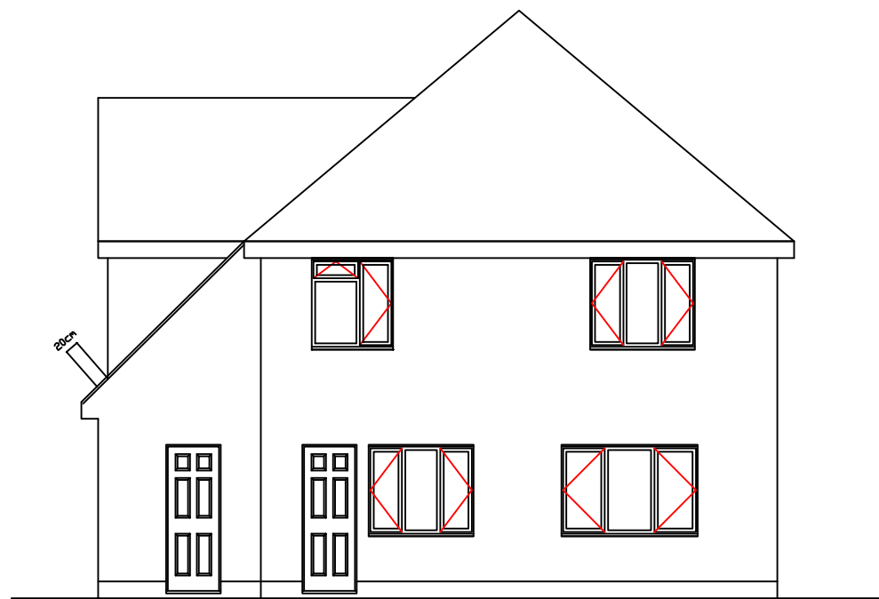
Rear
