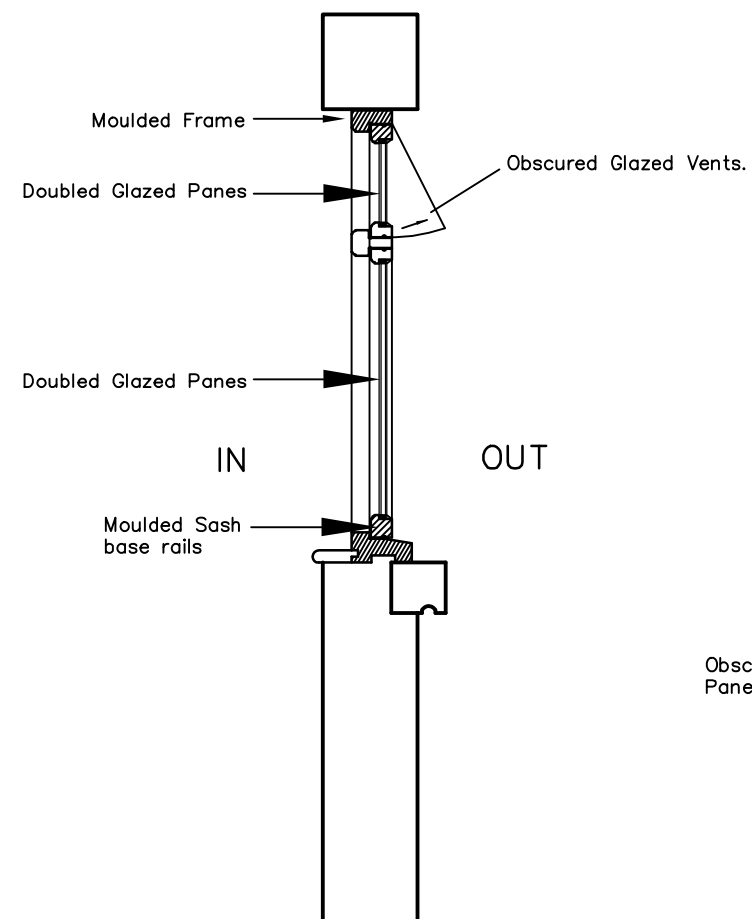
SECTION
