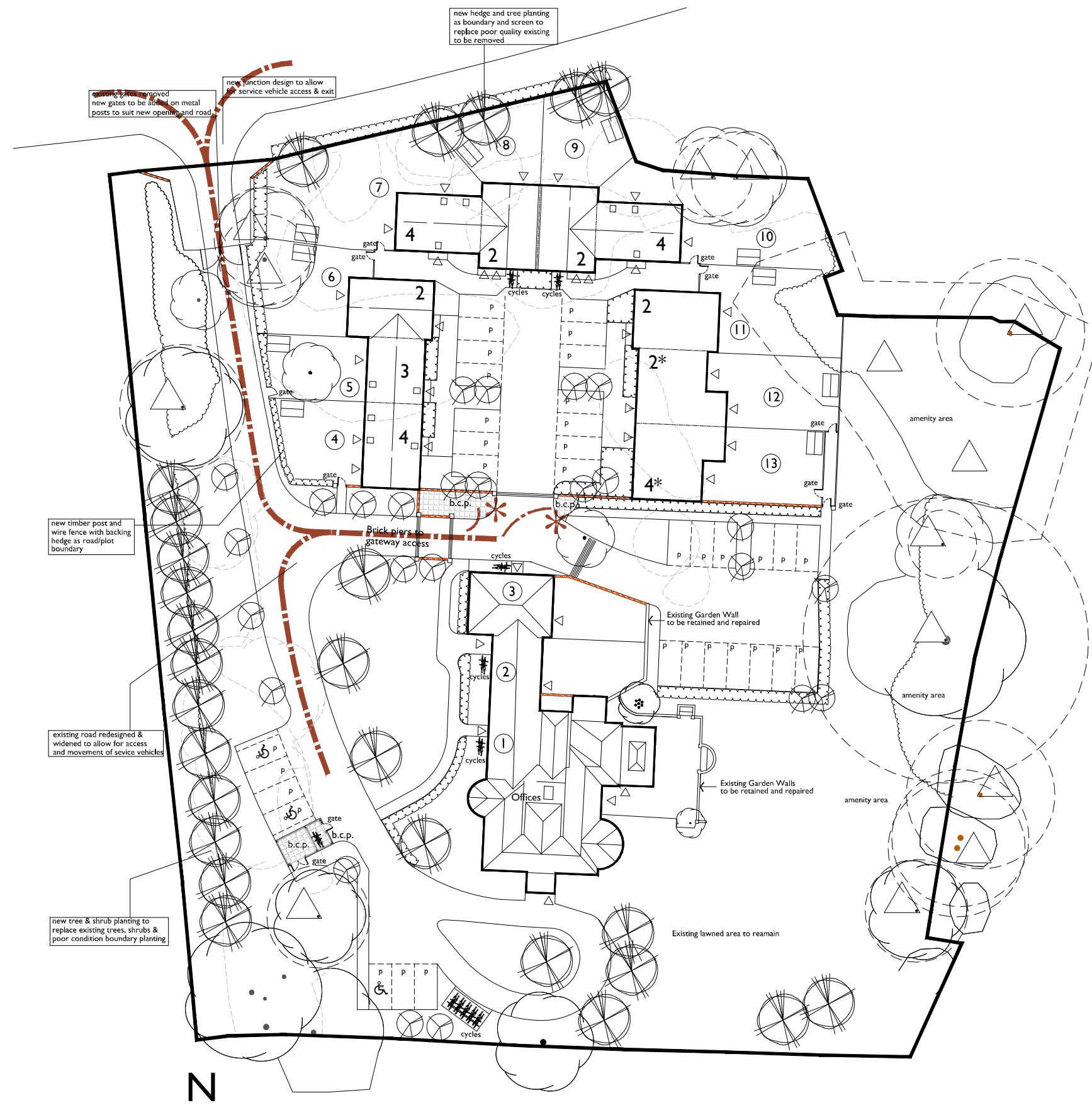
SITE PLAN : REFUSE VEHICLE ROUTE
