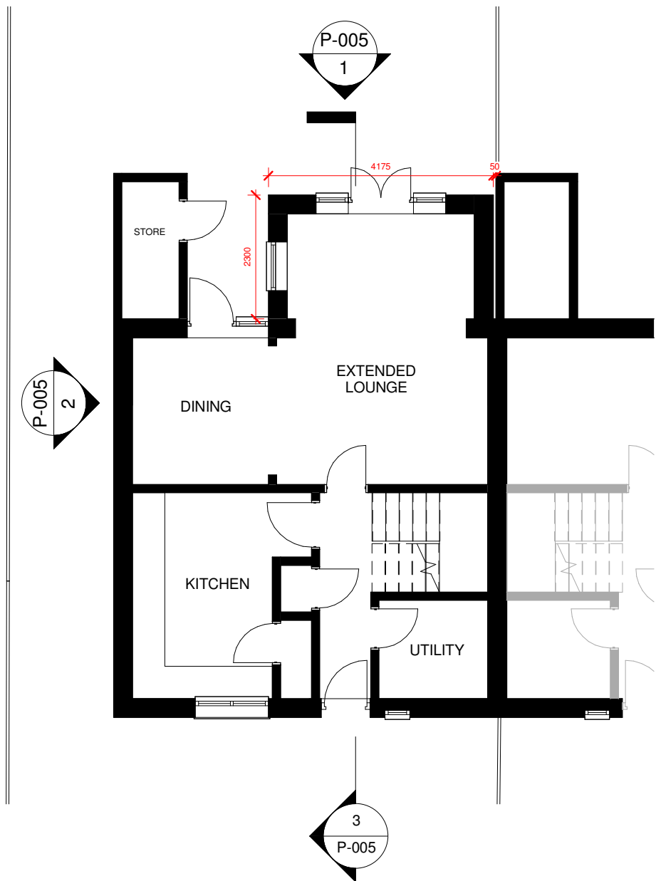
1 | P-004 PROPOSED GROUND FLOOR PLAN 1 : 100
