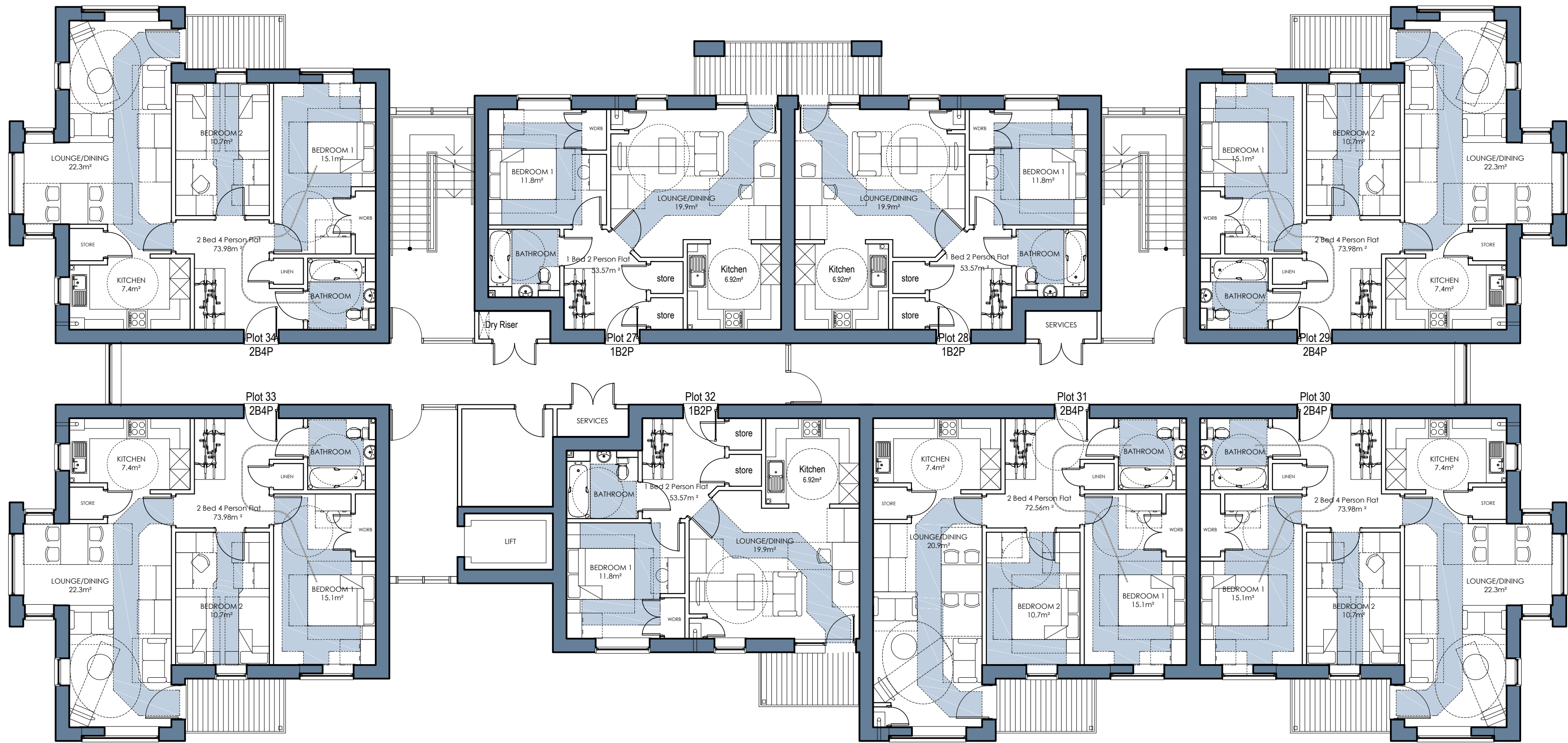
FIRST FLOOR
