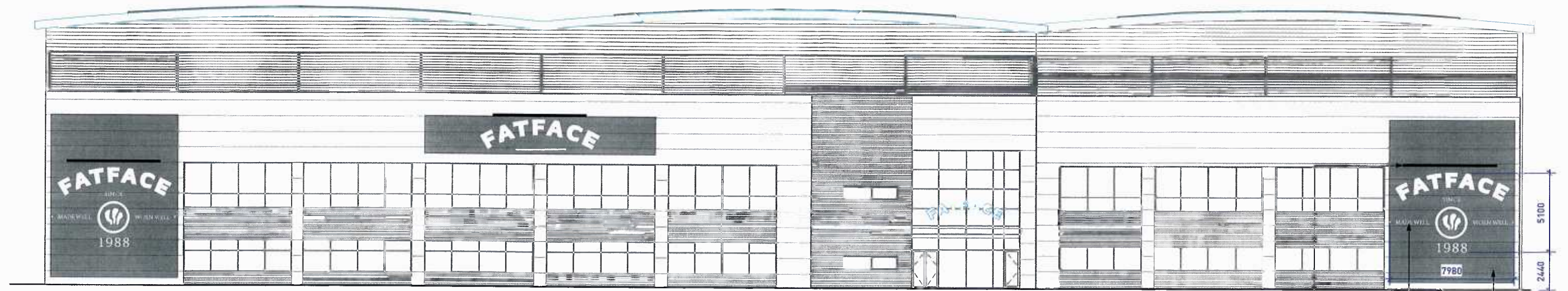
NORTH ELEVATION
