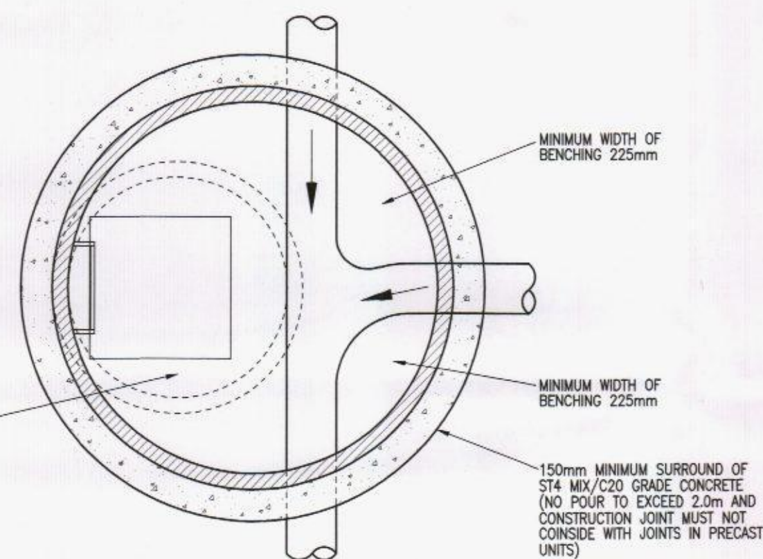
MANHOLE TYPE 2 UPTO 3.0m DEPTH
