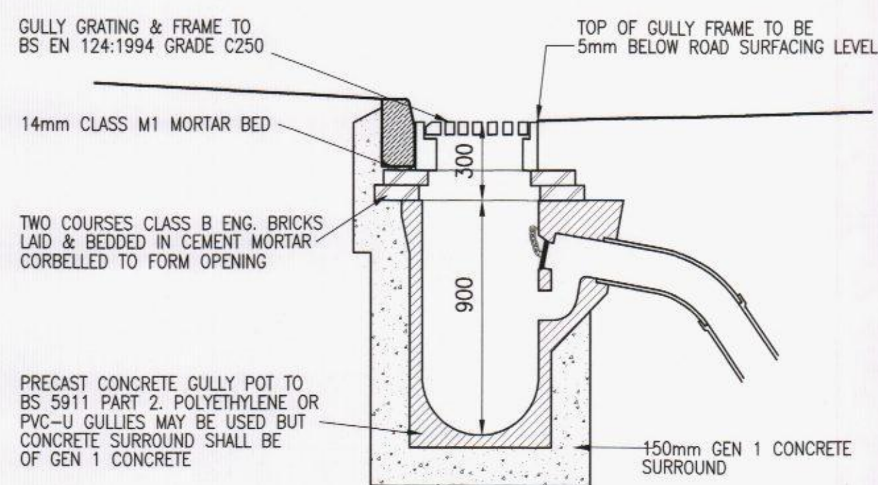
KERBSIDE ROAD GULLY
