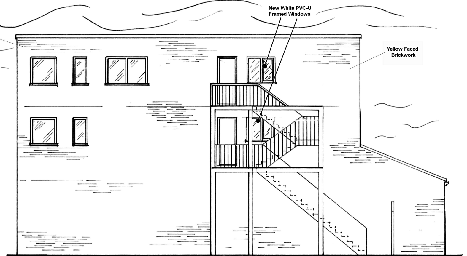
East Elevation
