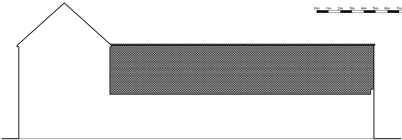
EXISTING WESTERN ELEVATION
