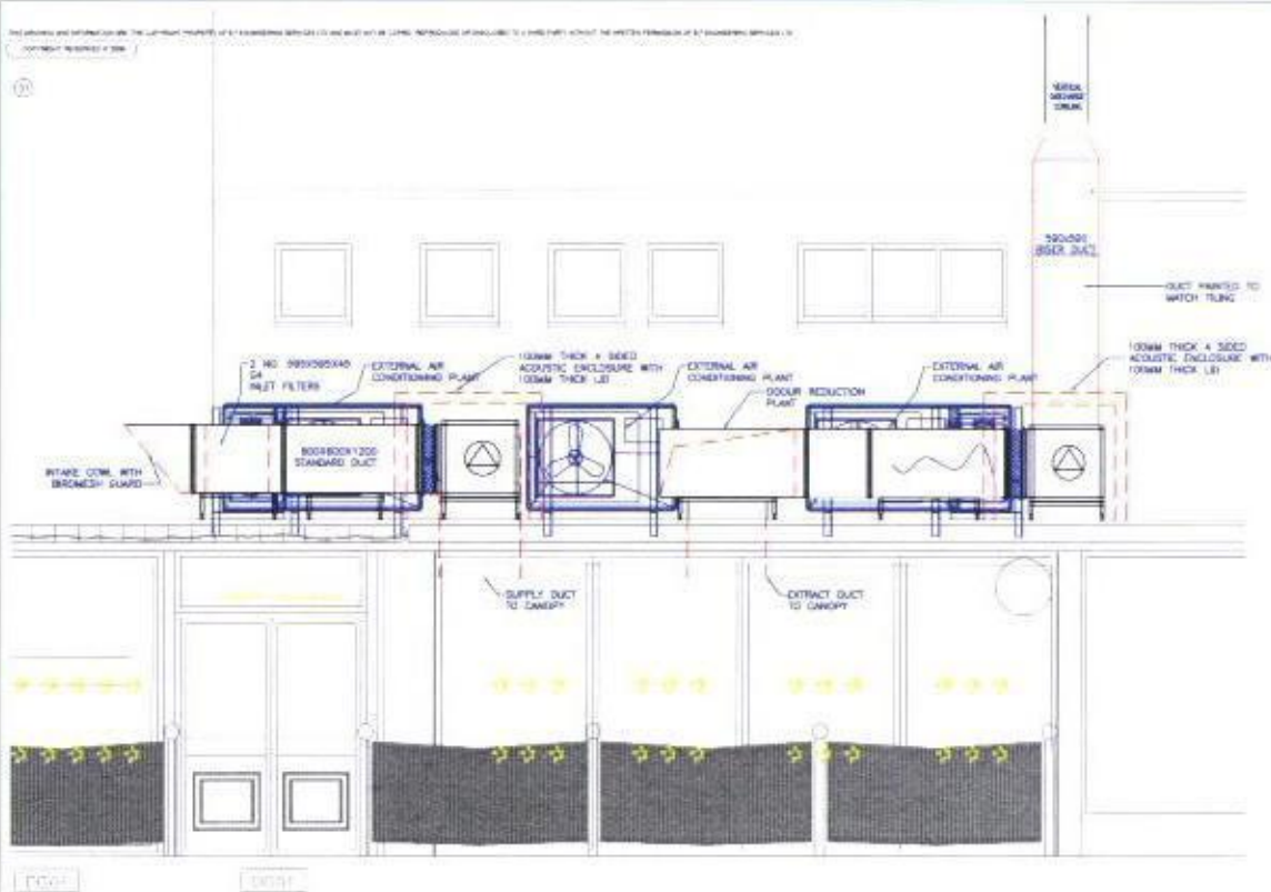
PROPOSED WEST SECTION
