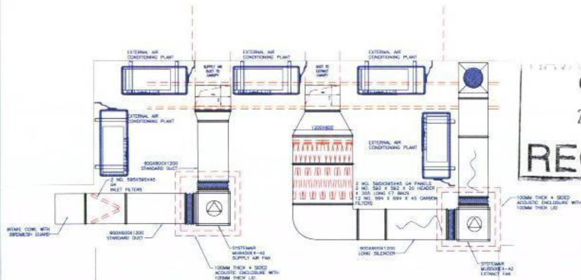
PLAN VIEW ROOFSIDE VENTILATION, ODOR REDUCTION AND ATTENUATION PLANT
