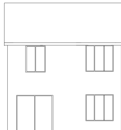
PROPOSED REAR ELEVATION (South no change)
