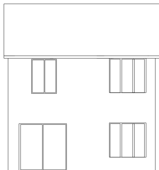
EXISTING REAR ELEVATION (South)
