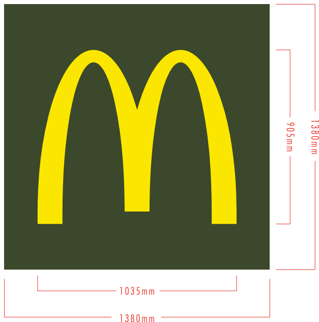
ARCH PANEL - scale 1:20
