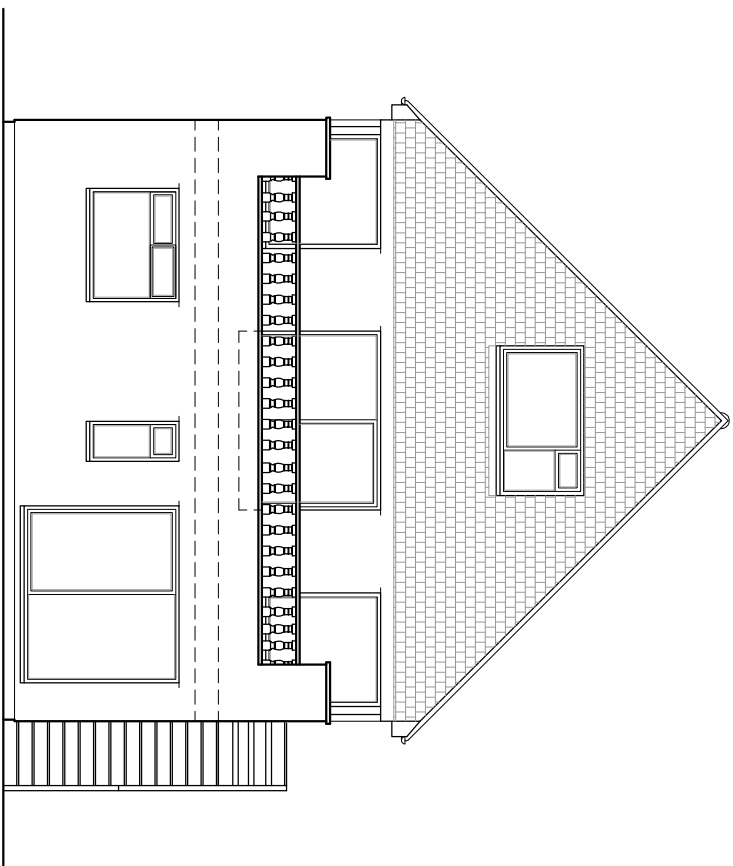
South (Rear) Elevation - As Existing
