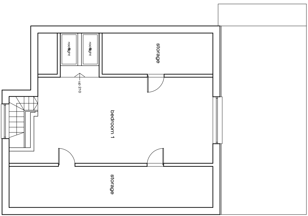
Second Floor Plan - As Existing
