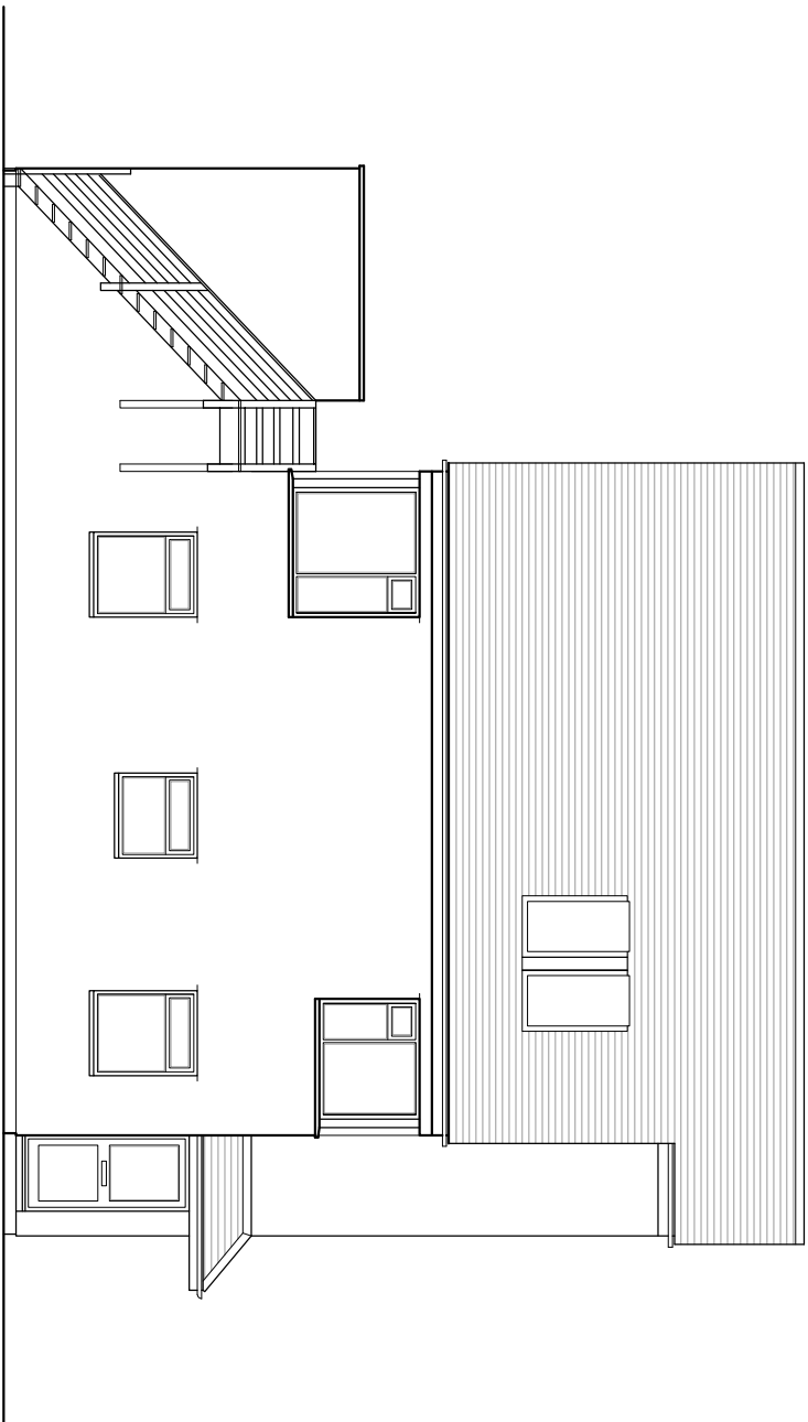
East (Side) Elevation - As Existing
