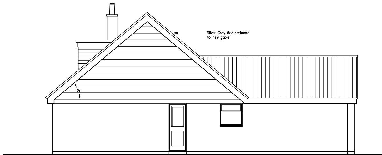
EAST FACING
