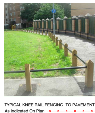
TYPICAL KNEE RAIL FENCING TO PAVEMENT As Indicated On Plan
