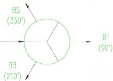
PROPOSED ANTENNA LAYOUT @ 12.24m SCALE 1:20
