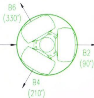
PROPOSED ANTENNA LAYOUT @ 10.37m SCALE 1:20
