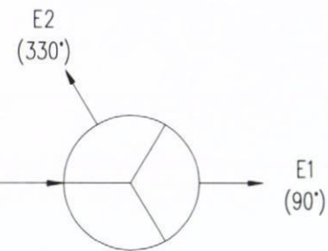
EXISTING VF ANTENNA LAYOUT @ 7.3m SCALE 1:20
