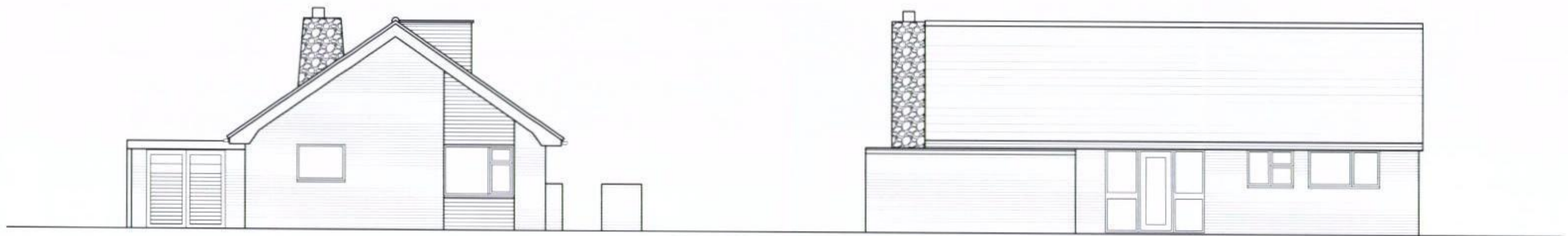
NORTH ELEVATION
