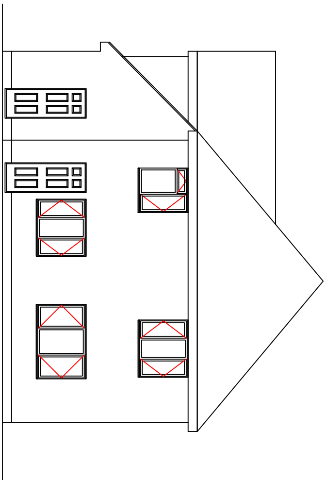
Rear
