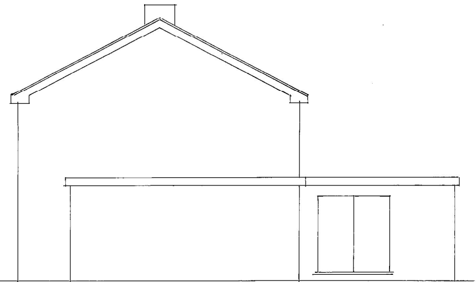
Existing South/Side Elevation
