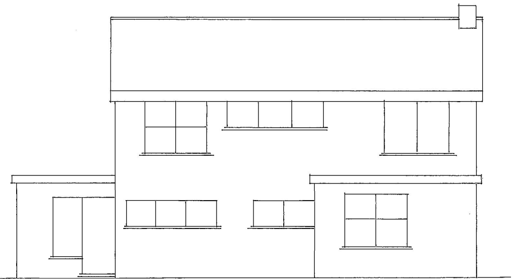
Existing East/Rear Elevation
