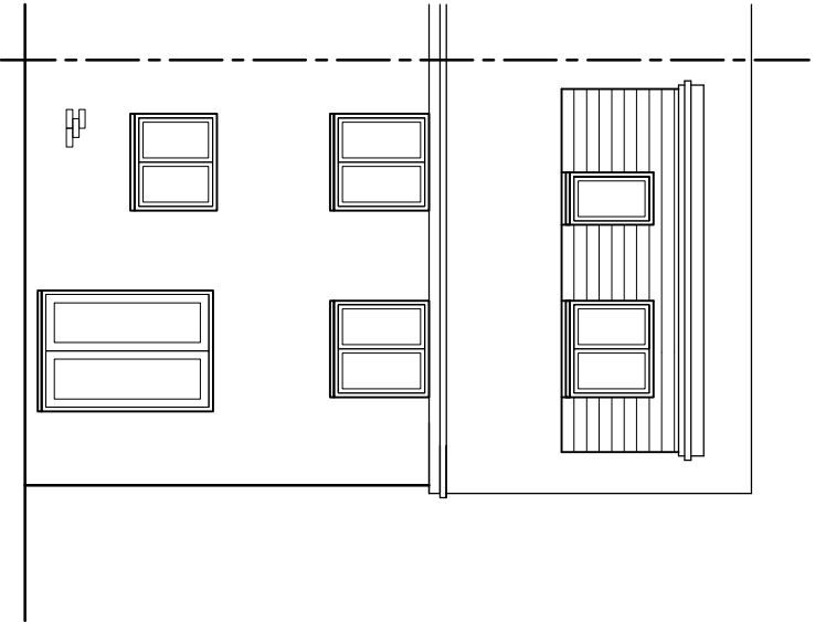
Rear 1:100
