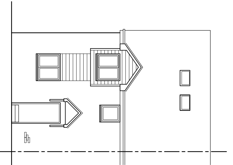
Front 1:100
