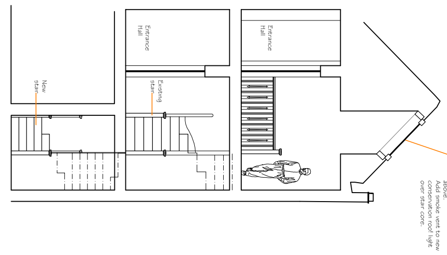
SECTION C-C
