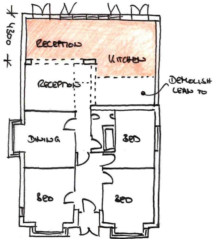
PROPOSED FLOOR PLAN - NTS
