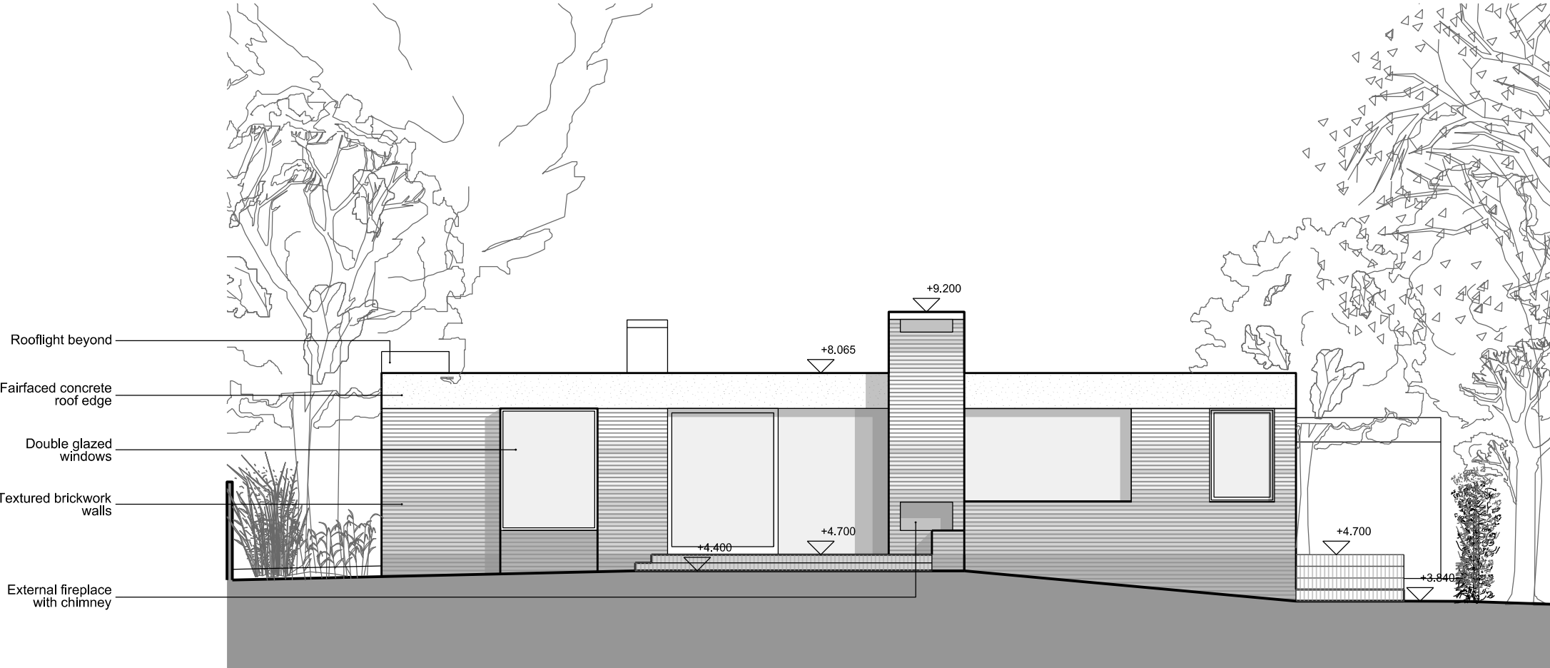
02 | NORTH ELEVATION PL09 |
