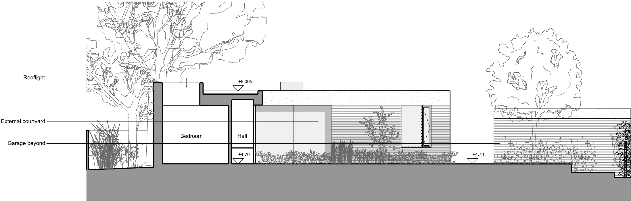
01 | NORTH INTERNAL COURTYARD ELEVATION PL09 |
