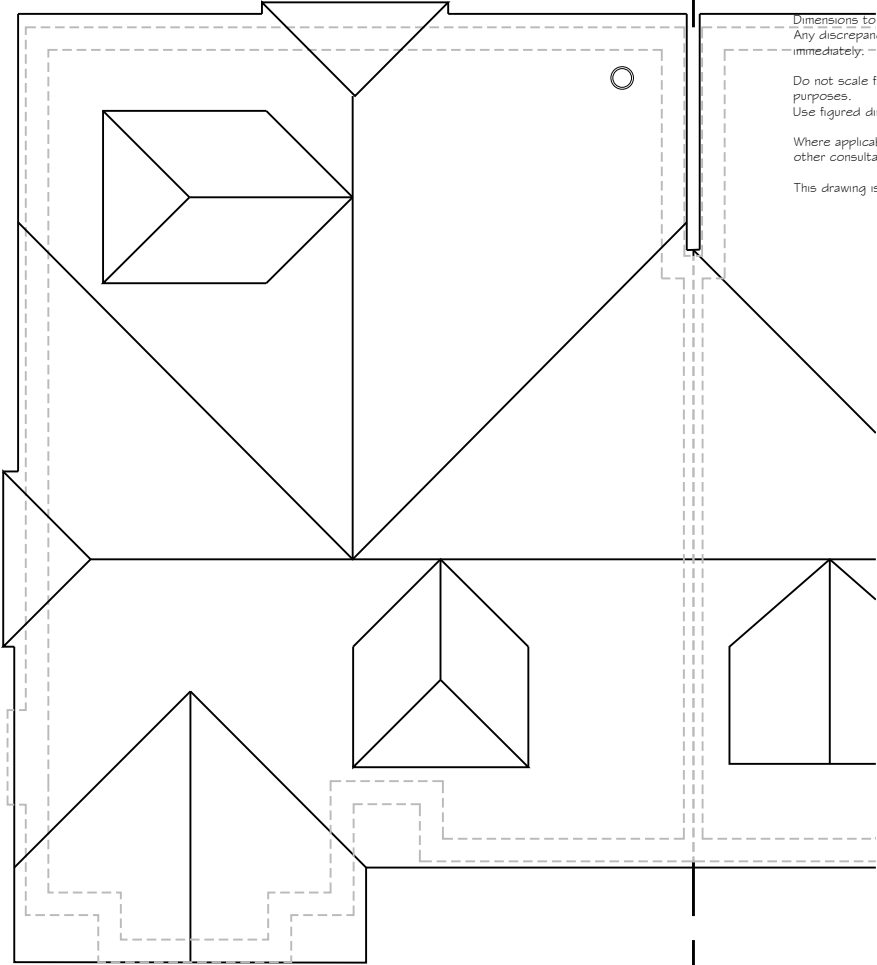
Roof Plan
