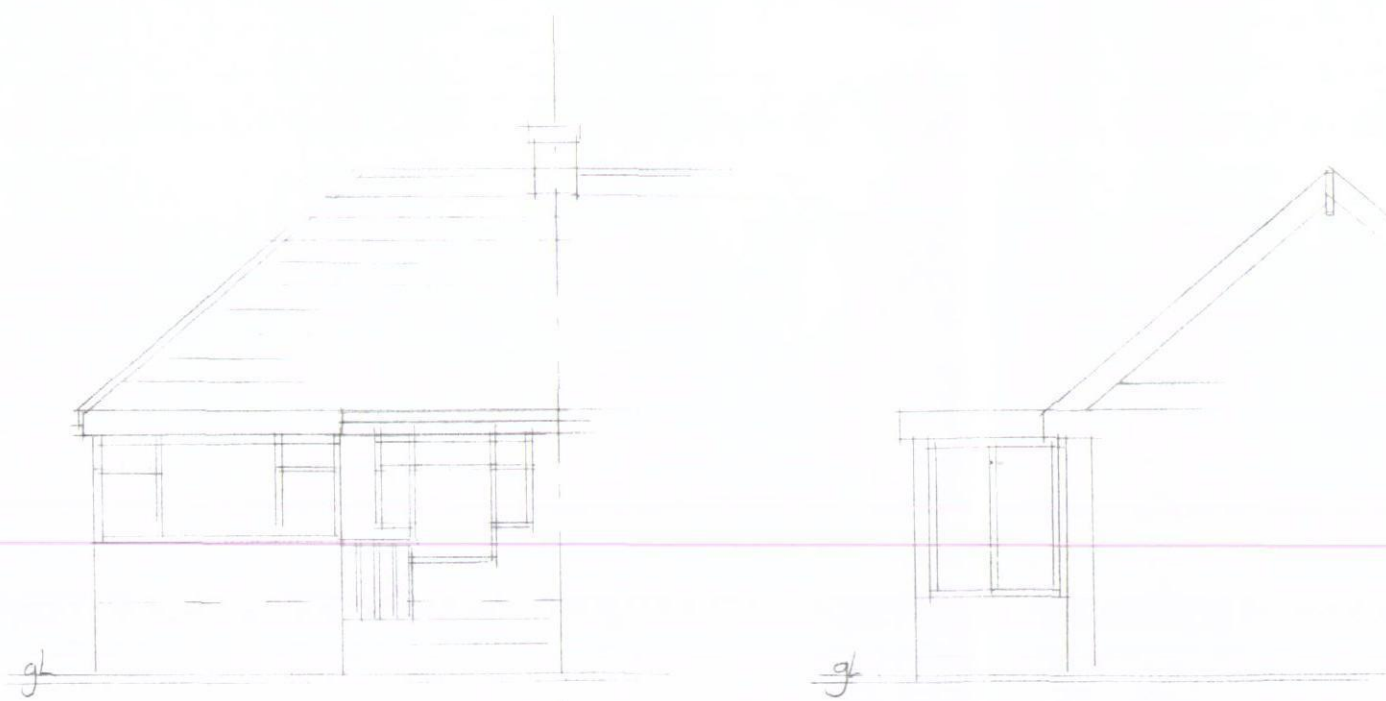
EXG SIDE ELEVATION 1:100
