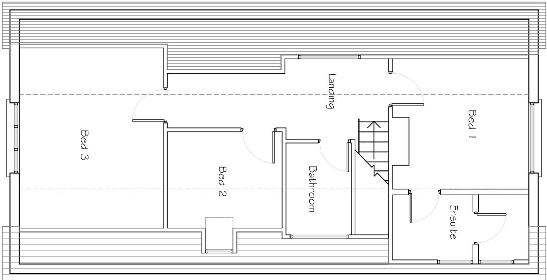
Existing First Floor Plan Scale 1:100
