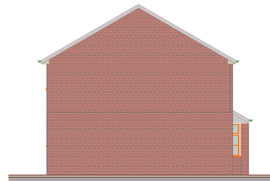
SW Elevation Existing 1:100
