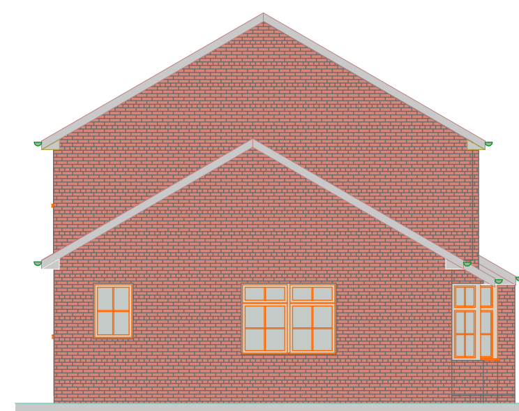
Proposed South West Elevation 1:100
