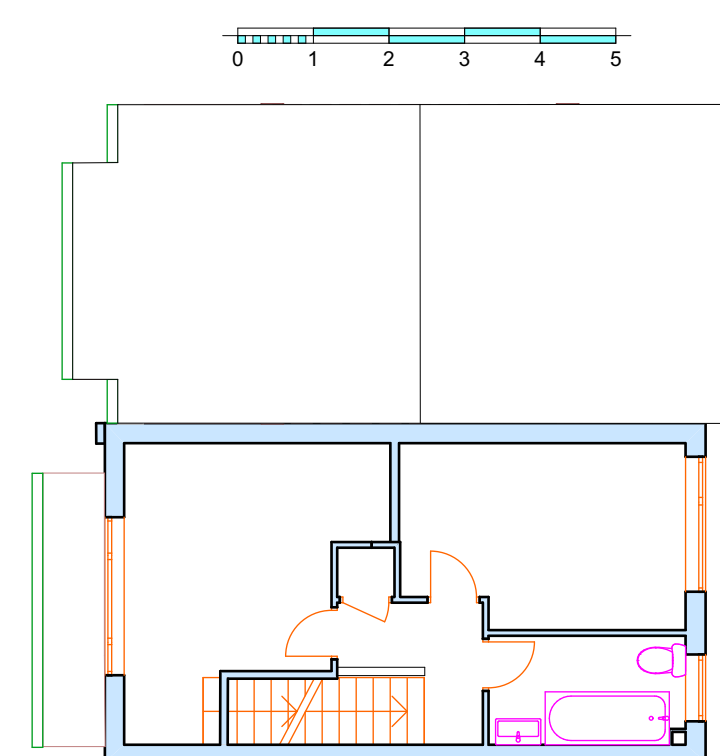
First Floor Unaltered 1:100
