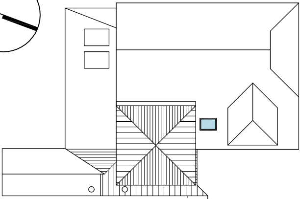
proposed roof plan 1:200
