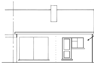
Proposed South/Rear Elevation
