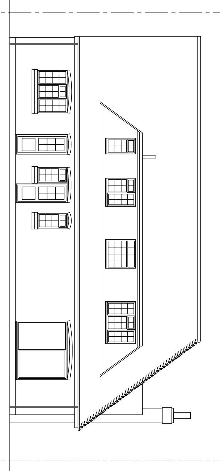
North Elevation
