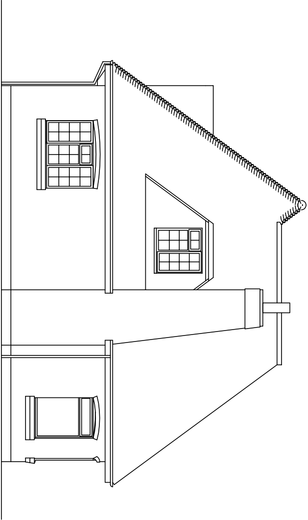
West Elevation
