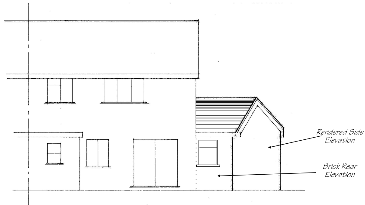
Proposed North/Rear Elevation
