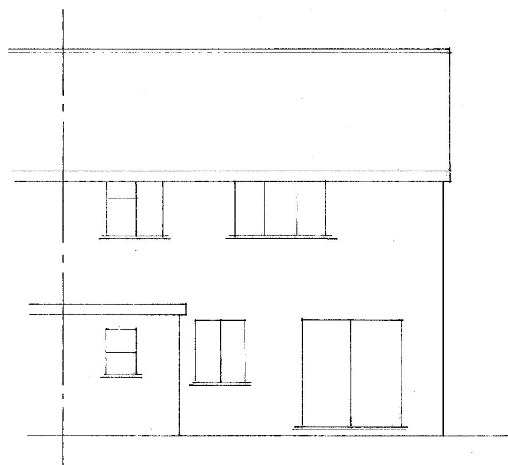
Existing North/Rear Elevation
