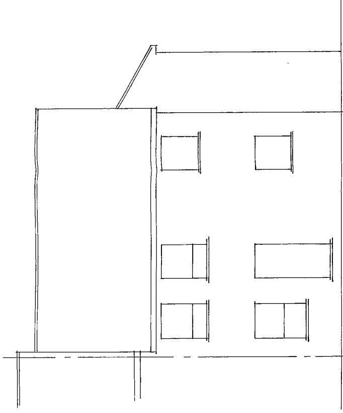
Existing West/Rear Elevation
