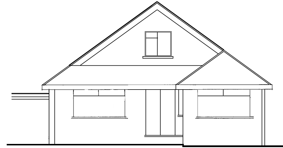
Proposed SE/Front Elevation
