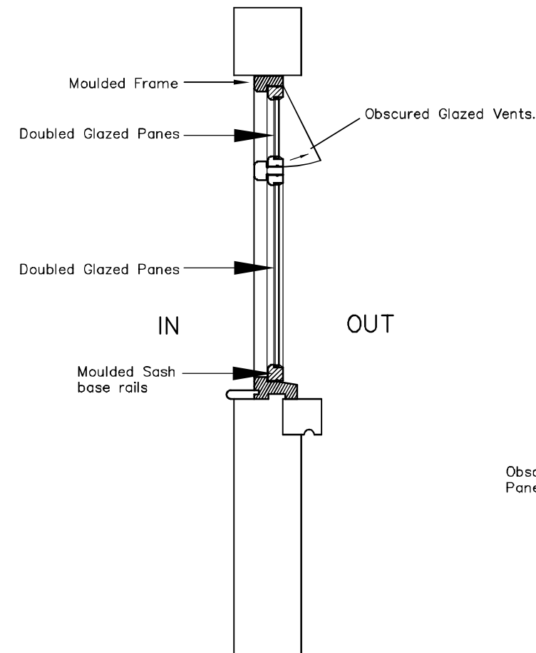
SECTION
